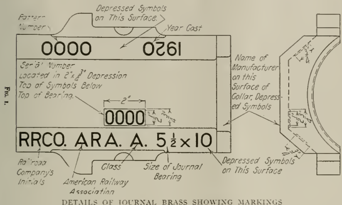
DETAILS OF JOURNAL BRASS SHOWING MARKINGS
